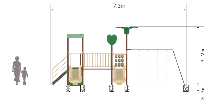
Vista frontal:
